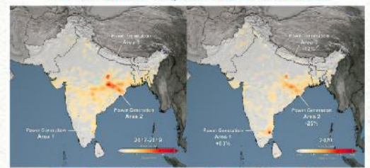
Pandemic Before and After Sulphur Dioxide data 2017-2019 versus 2020
