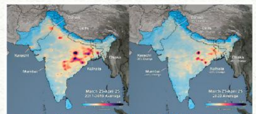
Pandemic Before and After Nitrogen Dioxide data 2017-2019 versus 2020
